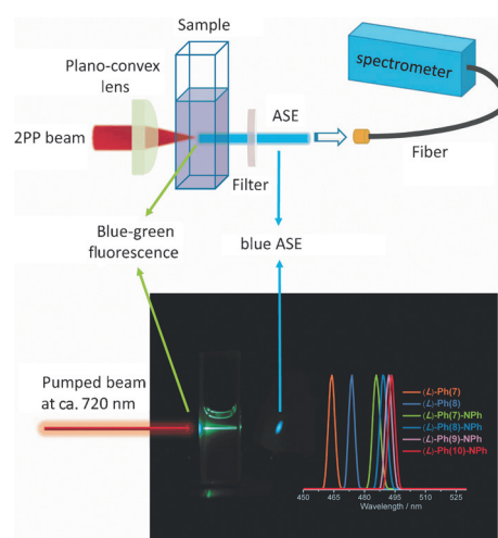
Figure 3. The 2PP ASE/lasing experimental setup for the measurement of the solution samples (top). Photo of highly directional, frequency-upconverted stimulated blue emission from a solution of ( L )-Ph(8)-NPh pumped at 720 nm fs laser beam (bottom). Inset: 2PP upconverted ASE spectra of ( L )-Ph( n ) ( n = 7, 8) and ( L )-Ph( n )-NPh ( n = 7–10).
